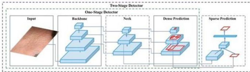
Fig.5. Object detectors that are one stage or two stages differ from each other.
