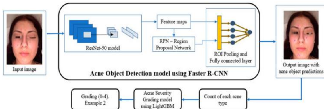
Fig.6. Faster R-CNN-based implementation of appropriate activity recognition model.
