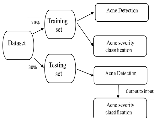
Fig.3. Skin conditions prediction dataset equally distributed for testing/training.
